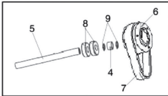
Conjunto soporte cuchilla Blade support set Ensemble support lame
